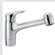
Single-lever mixer with swivel spout, with pull-out hand shower 0138 2273 chrome 0138 2273 82 white 0136 1173 chrome †
