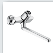
Wall-mounted single-lever mixer with swivel spout, 300 mm, without lever 0369 2100 chrome with shut-off S-connections, 311 mm, without lever 0369 2200 chrome
